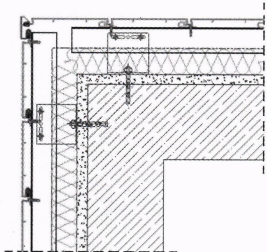
8 DAMLALIK DETAYI 1
