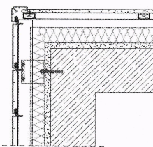
9 DAMLALIK DETAYI 2
