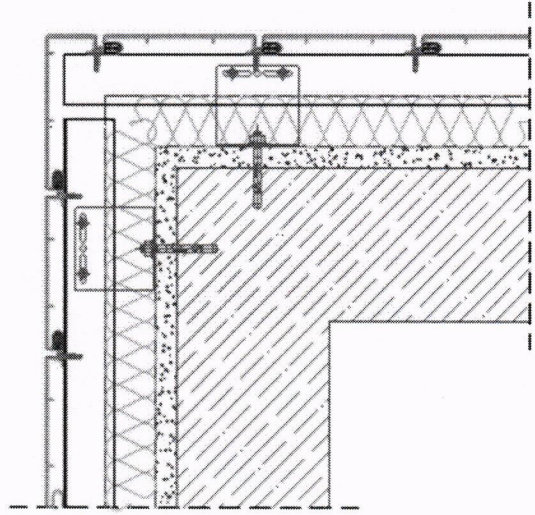
10 DAMLALIK DETAYI 3
